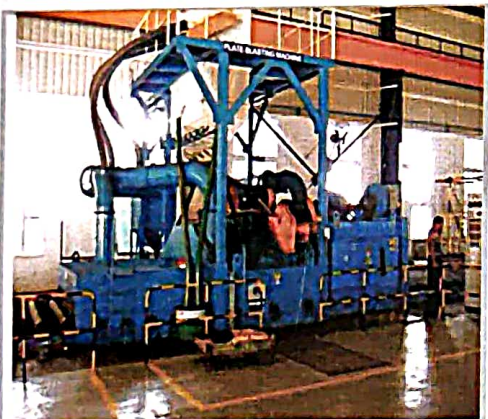
Tunnel Type 8 Wheel Shot Blasting M/c for Plate Cleaning
