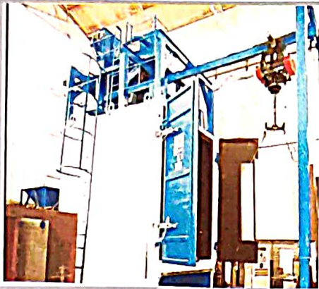
'T' Hanger Type Shot Blasting M/c with Motorized Hoist
