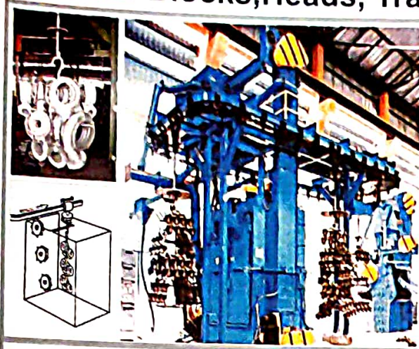
2 Wheel Continues Monorail & Hanger Machine, Capacity : 4 Hook 750 Kg, 800 Kg per Hanger
