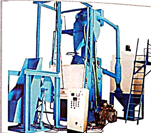
Airless Tumblast Type Shot Blasting M/c with Haydraulic Loader ATB-27x36
