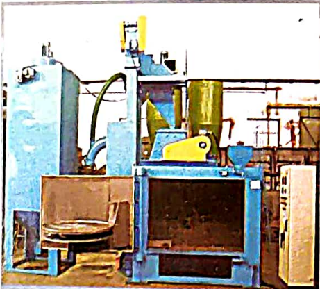
Single Door Type Swing Table Shot Blasting M/c
