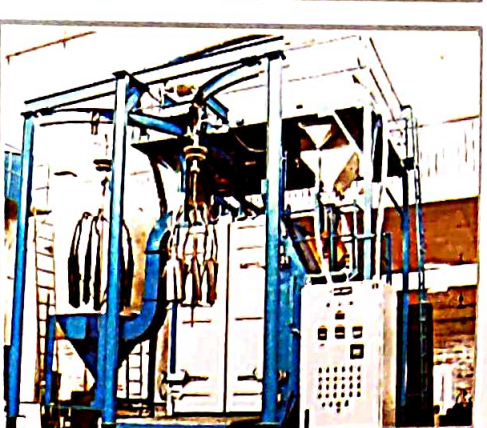
'Y' Hanger Type Shot Blasting M/c for Automobile Mufflers
