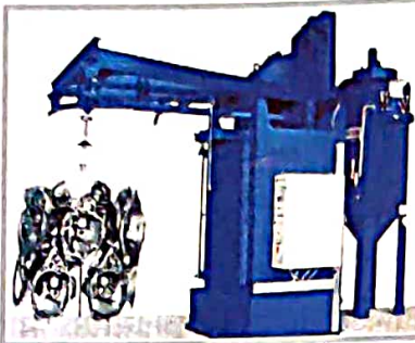
2 Wheel Y Type Hanger Machine Capacity : 500 Kg., 2000 Kg
