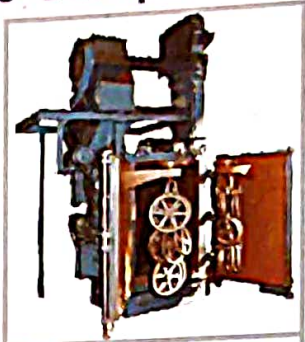
1/2 Wheel Door Hanger Machine Capacity : 100 / 500 Kg.
