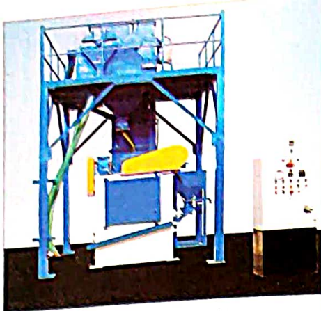
Airless Tumblast Type Shot Blasting M/c ATB-20x27
