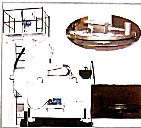
Double Door Type Swing Table Shot Blasting M/c MODEL : AST - 1600
