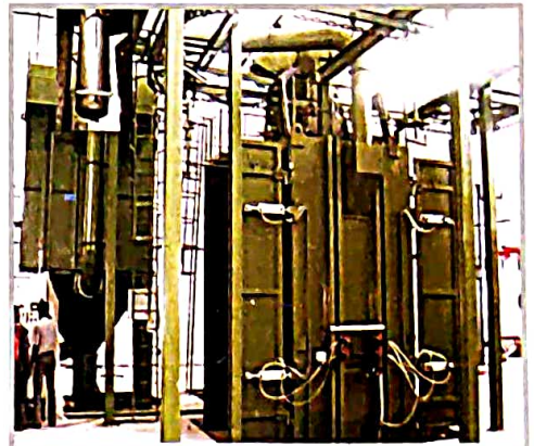
Continuous Monorail Hanger Loop Type Shot Blasting M/c
