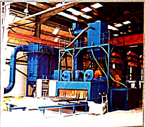
Tunnel Type 6 Wheel Shot Blasting M/c for Plate Cleaning M/c
