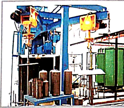
'Y' Hanger type Shot Blasting M/c for Fire Extinguisher Cylinder
